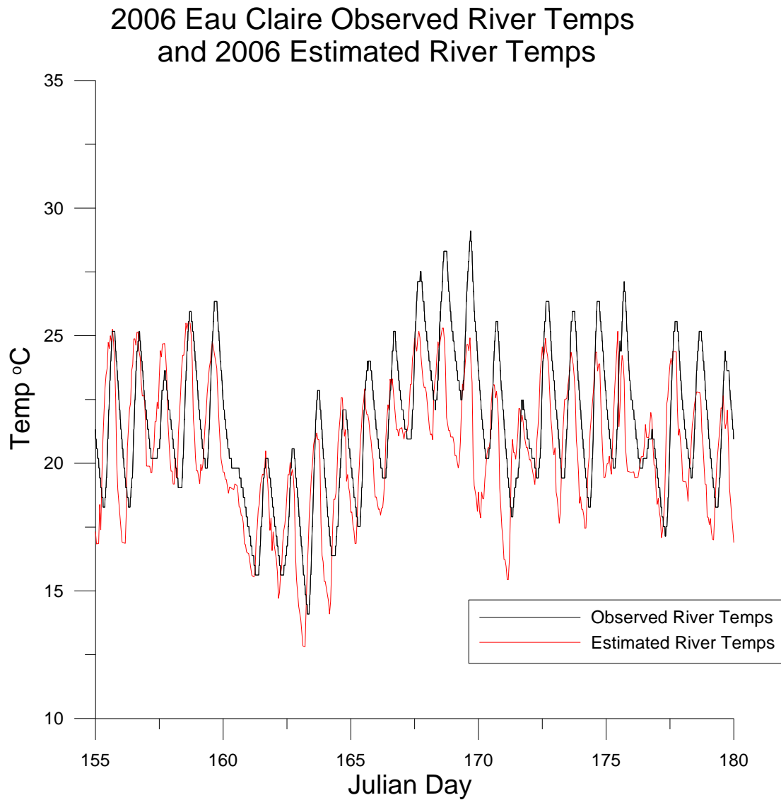
Figure 5 Observed Eau Claire River Temperatures and estimated River Temperatures using Equation 1.
