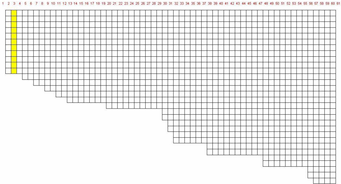
Figure 4 Side view of the Lake Eau Claire CE-Qual-W2 model
