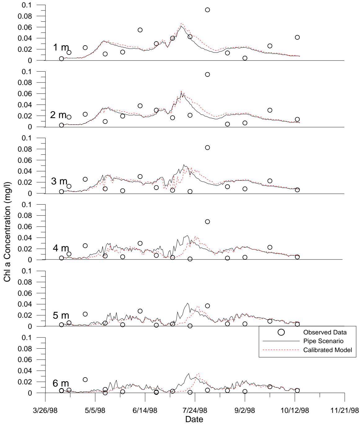
Figure 15 1998 CHL a Model Calibration and Pipe Scenario vs. Observed Data by Depth - Segment 41
