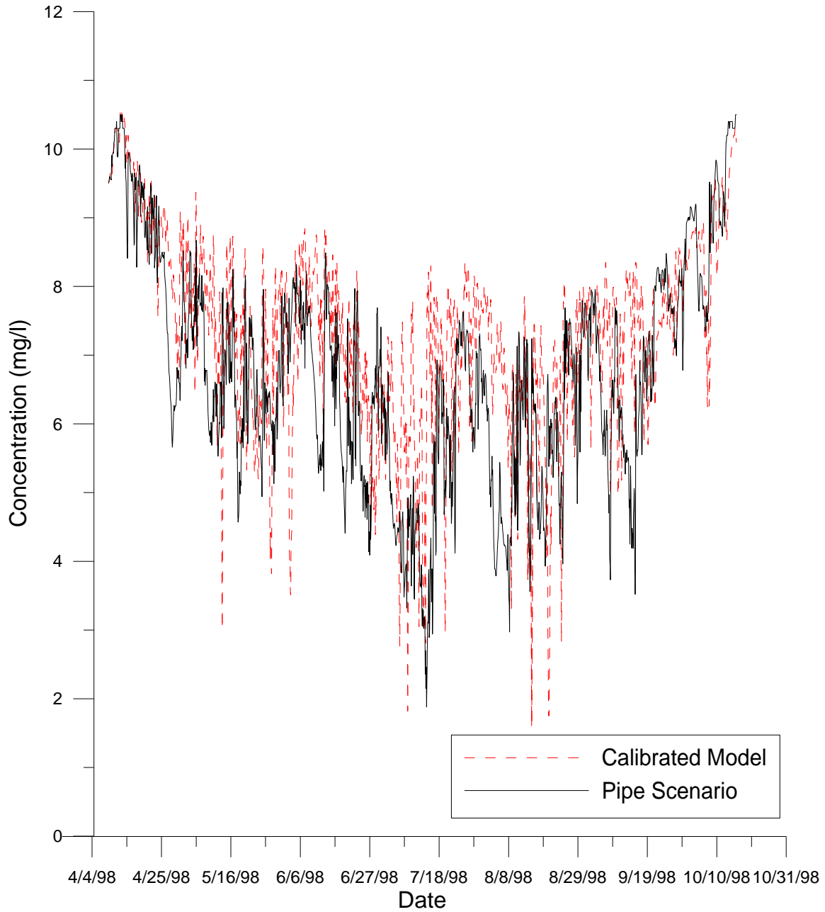
Figure 17 1998 Dam Outflow - Calibrated Model and Pipe Scenario D.O. Concentrations
