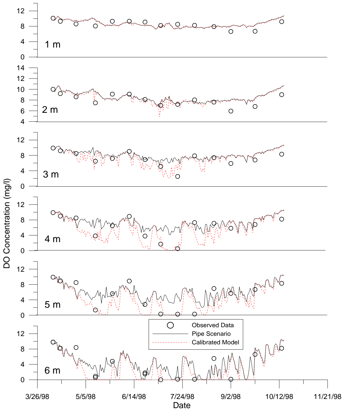
Figure 11 1998 DO Model Calibration and Pipe Scenario vs. Observed Data by Depth - Segment 41
