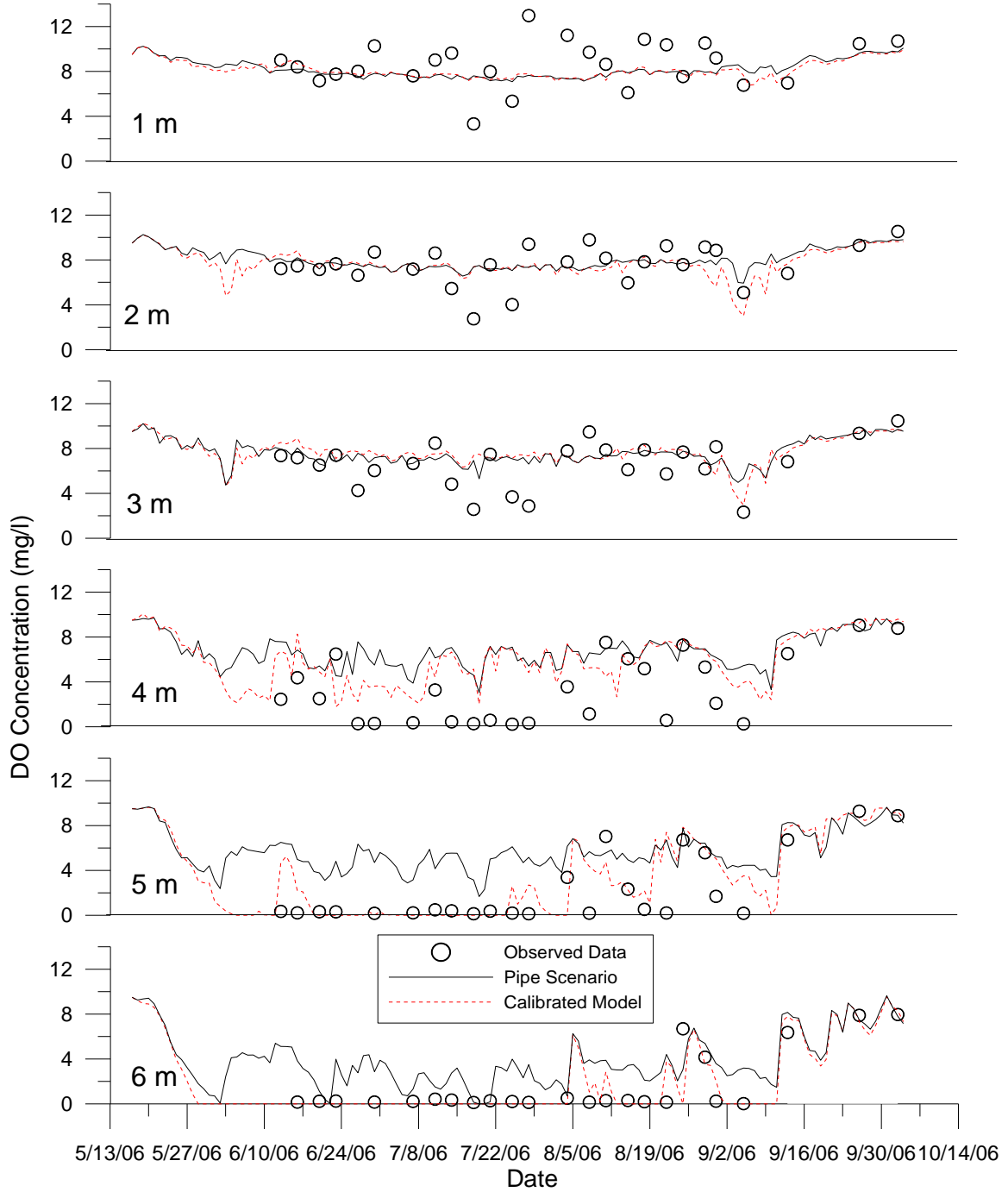
Figure 12 2006 DO Model Calibration and Pipe Scenario vs. Observed Data by Depth - Segment 49
