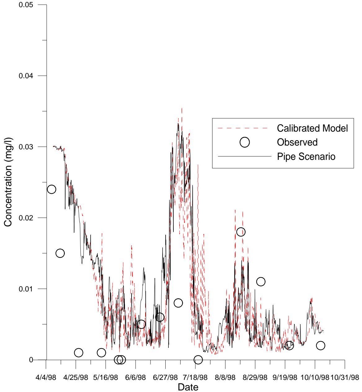
Figure 18 1998 Dam Outflow - Observed SRP vs. Calibrated Model and Pipe Scenario PO4 Concentrations
