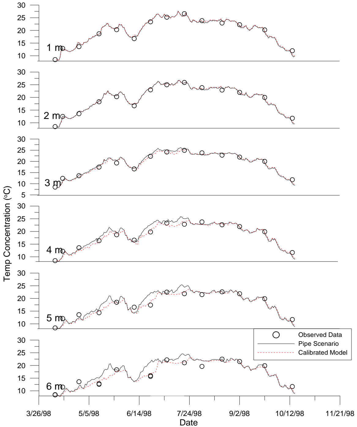
Figure 9 1998 Temp Model Calibration and Pipe Scenario vs. Observed Data by Depth - Segment 41
