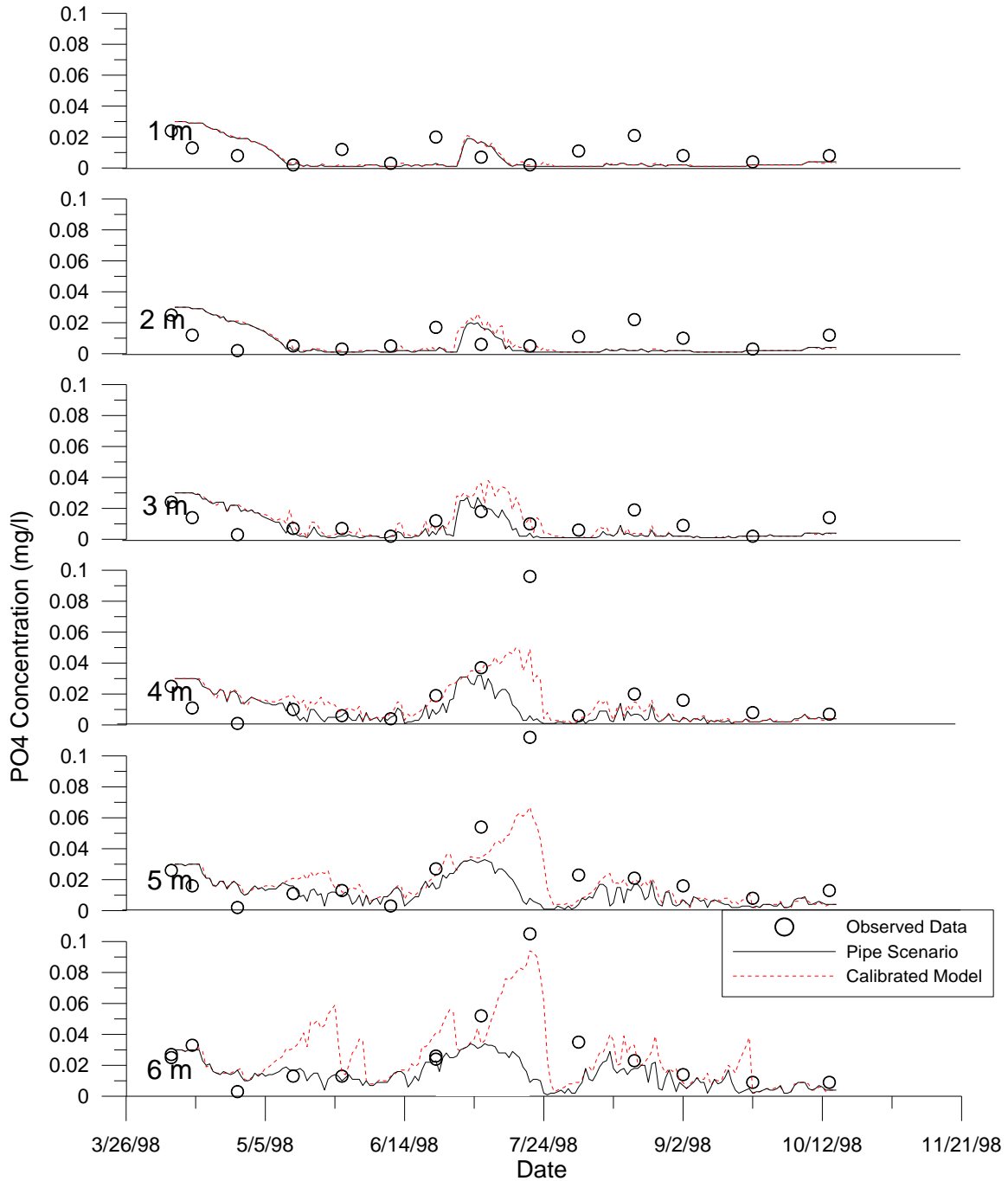
Figure 13 1998 PO4 Model Calibration and Pipe Scenario vs. Observed Data by Depth - Segment 41
