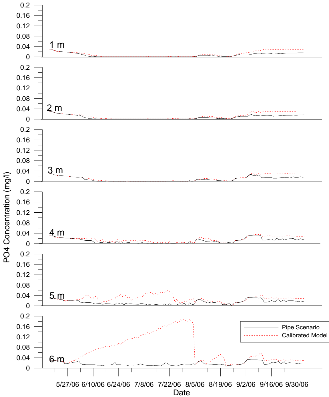
Figure 14 2006 PO4 Model Calibration and Pipe Scenario by Depth - Segment 49
