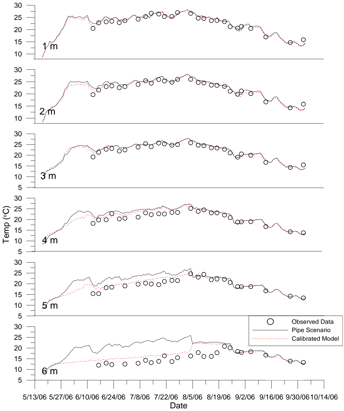
Figure 10 2006 Temp Model Calibration and Pipe Scenario vs. Observed Data by Depth - Segment 49
