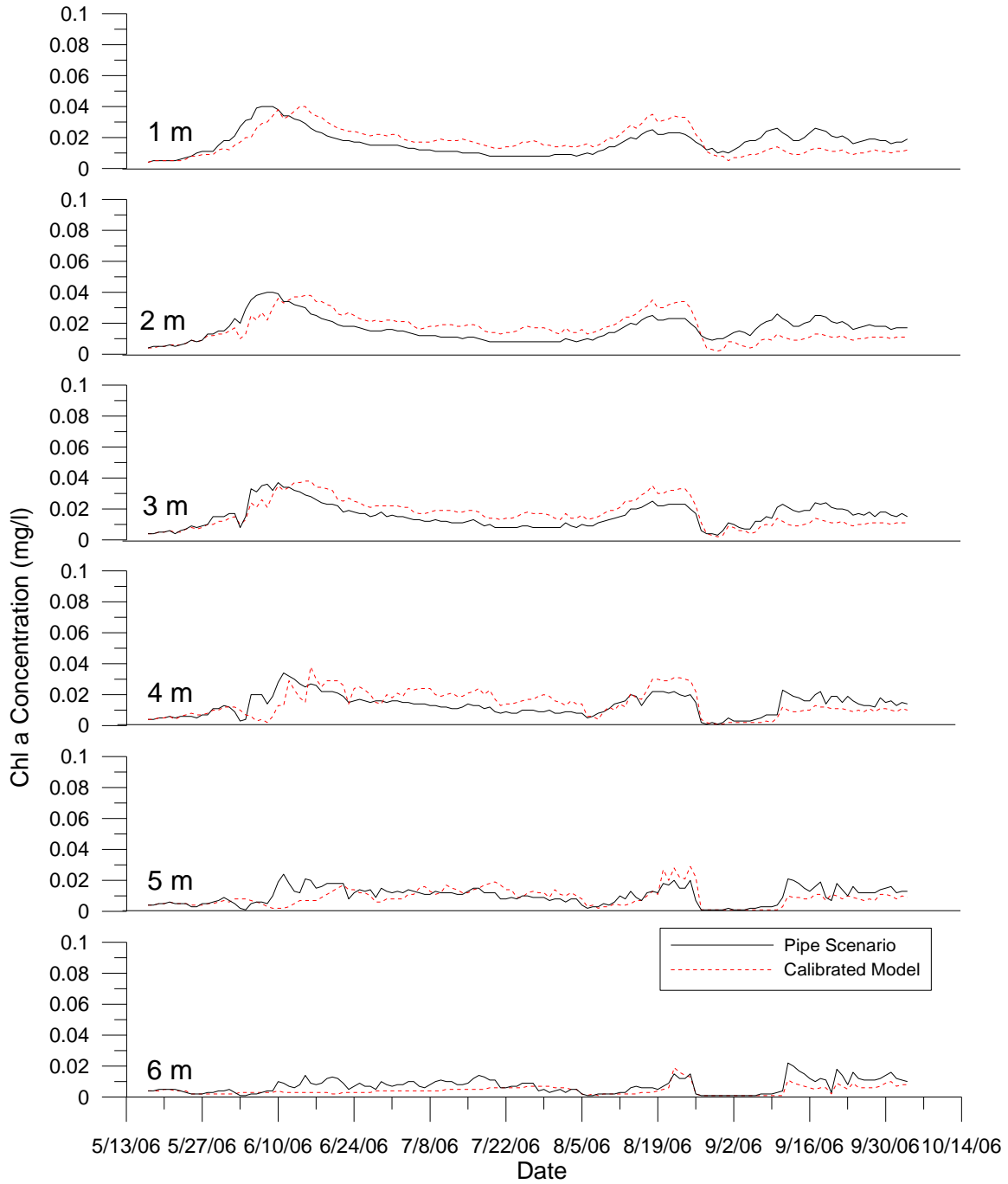
Figure 16 2006 Chl a Model Calibration and Pipe Scenario by Depth - Segment 49
